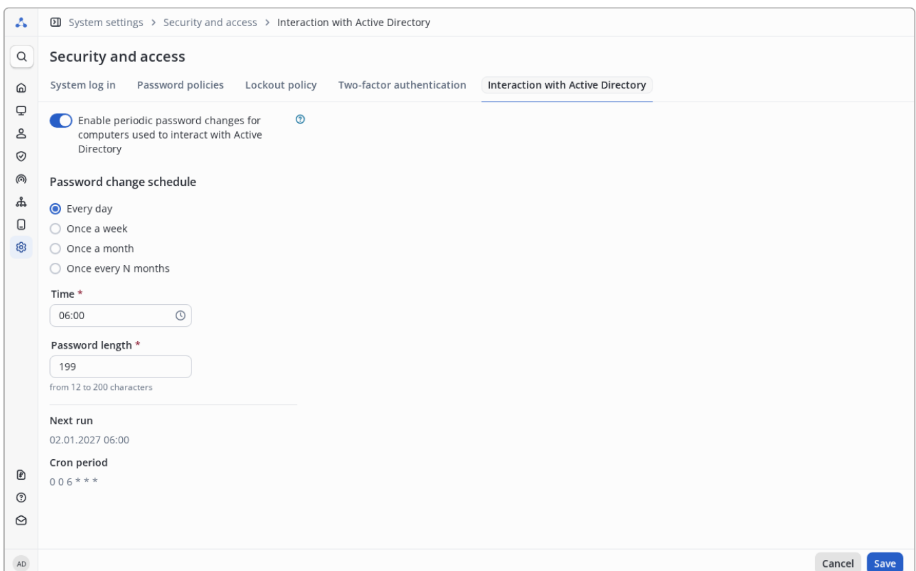
Figure 419. Password change schedule
