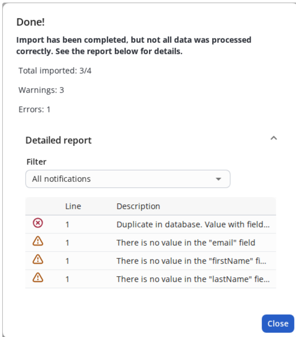
Figure 96. Window Import report (entries processed with errors/warnings)
