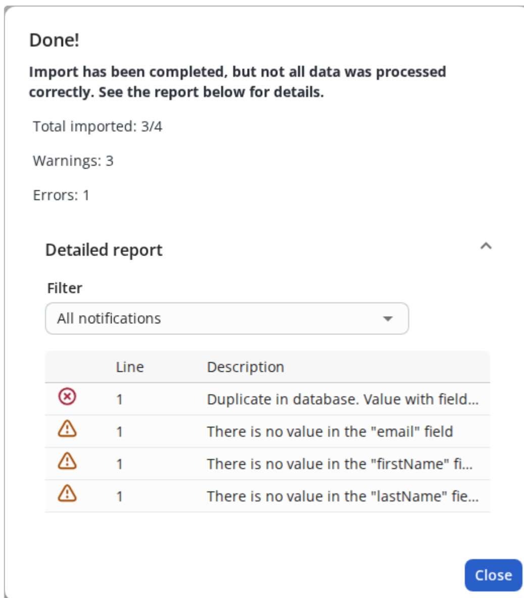
Figure 122. Window Import report (entries processed with errors/warnings)
