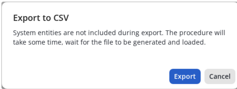
Figure 176. Export all
