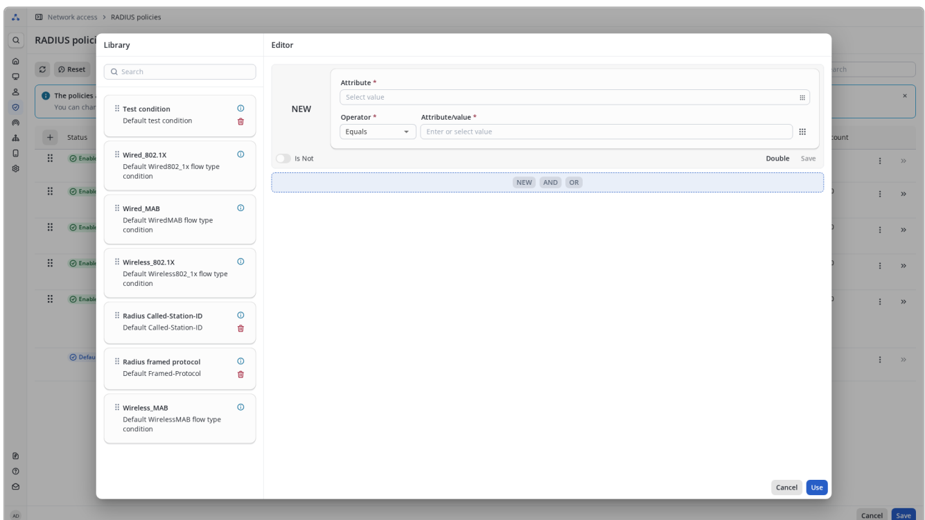
Figure 276. Conditions editor
