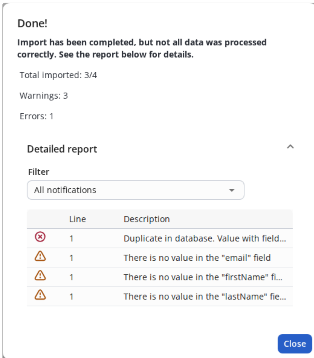
Figure 161. Window Import report (entries processed with errors/warnings)
