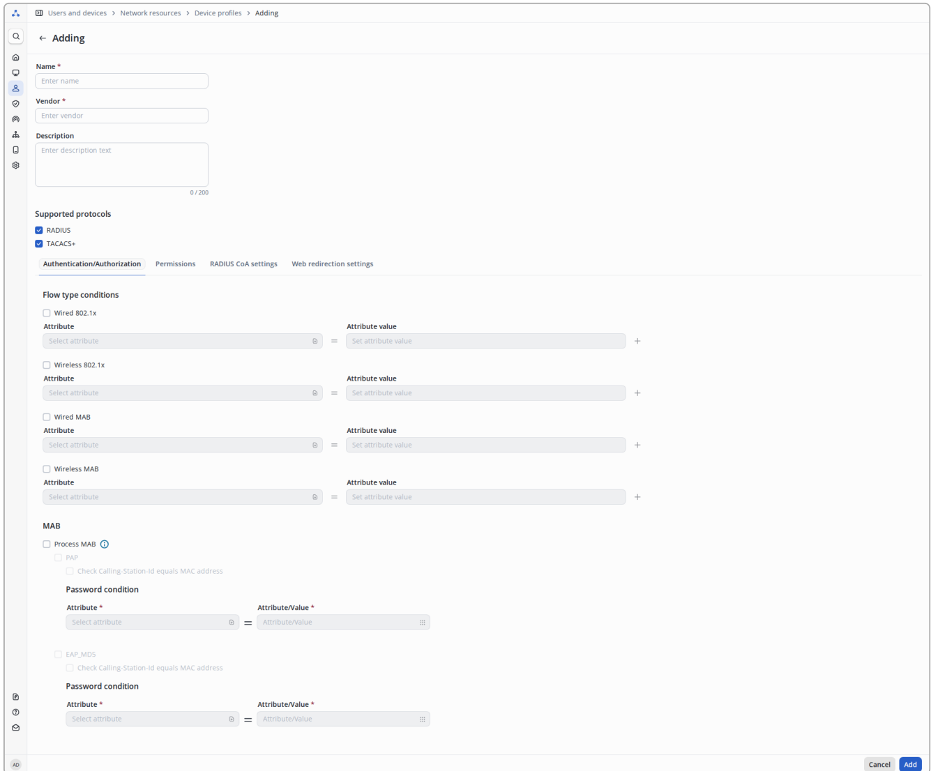
Figure 142. Page with filling device profile parameters. The Authentication/Authorization tab
