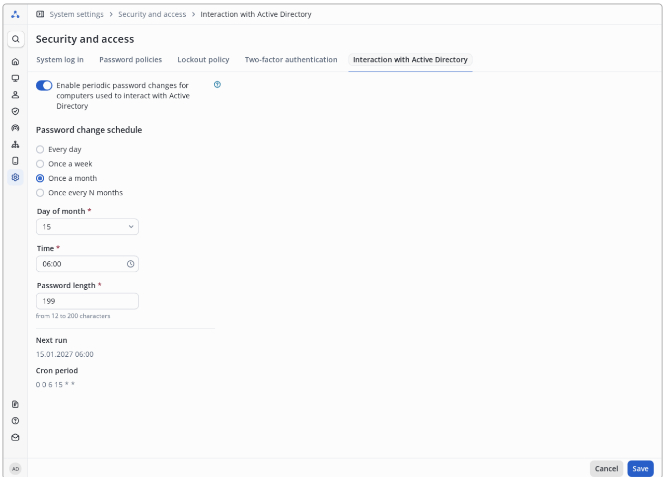
Figure 421. Password change schedule - monthly
