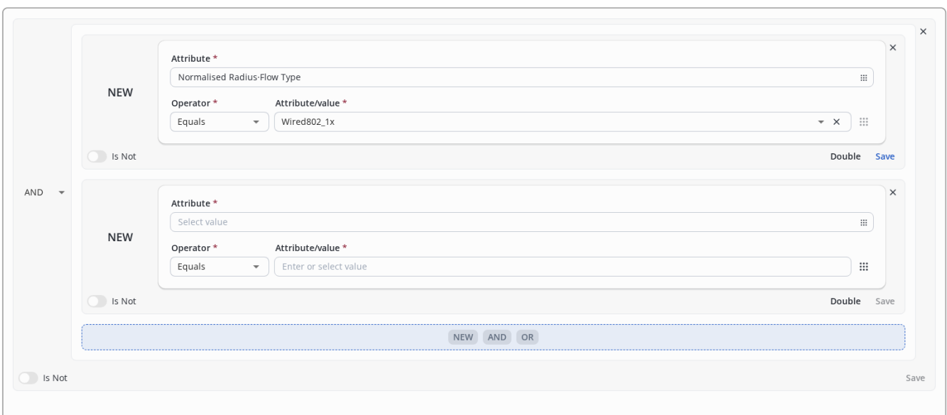
Figure 262. Condition consisting of two conditions combined by a logical "AND"
