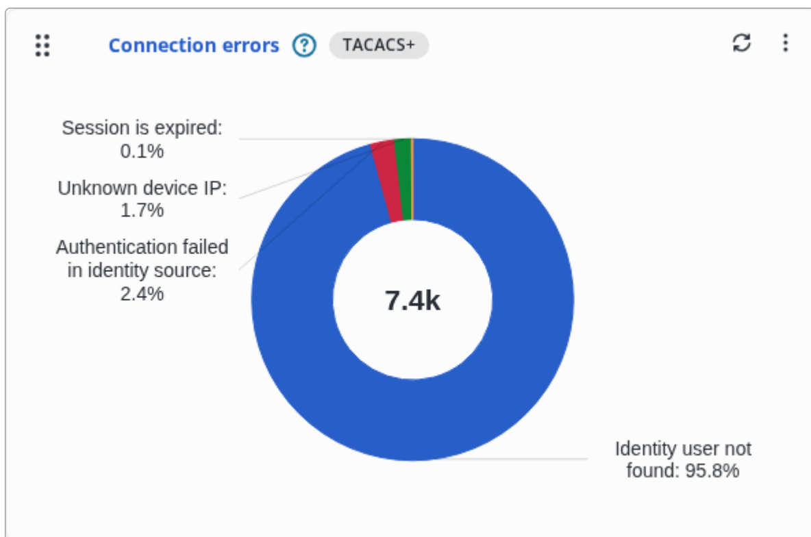
Figure 27. Widget "Connection errors"
