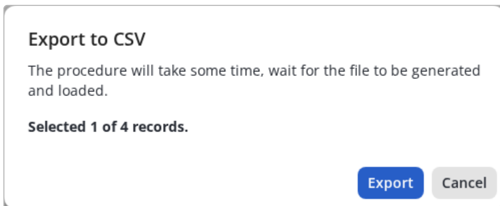
Figure 99. Export selected
